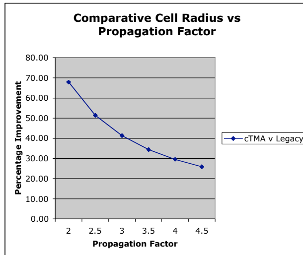
Fig. 2: cTMA Cell Radius Improvement vs \gamma
