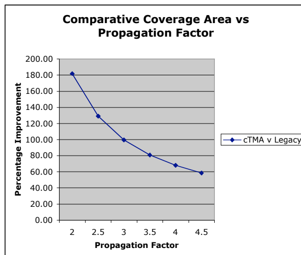
Fig. 3: cTMA Improvement in Cell Area vs \gamma
